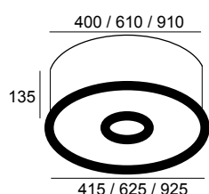
LED
