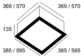
Diffusor
