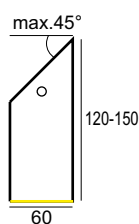
Cube AS
